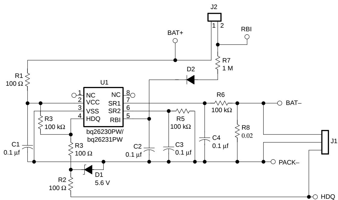
Figure 2–1. bq26231EVM-001 Schematic
